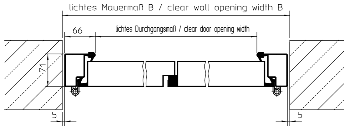
Stockrahmen stock frame
